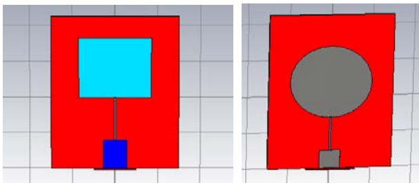
(a) Rectangular Patch (b) Circular Patch
