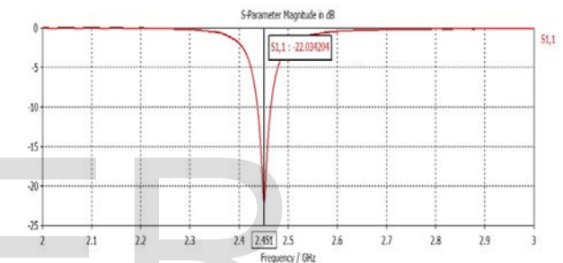
Fig. 3. Return loss response of Circular Patch Antenna.
