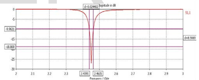
Fig. 4. Bandwidth calculation for Rectangular Patch Antenna
