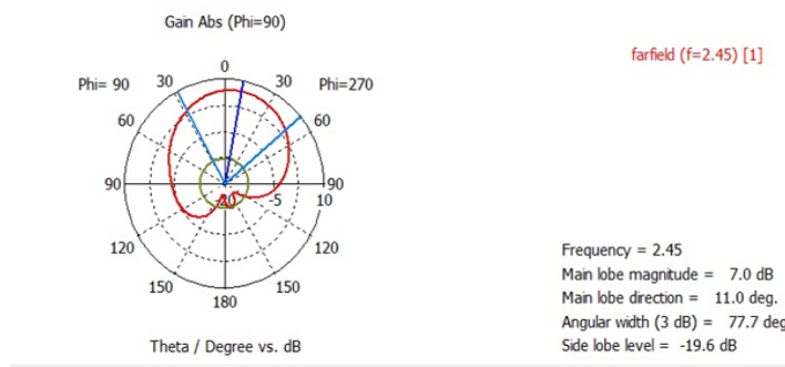
Fig. 8. Polar plot radiation pattern of Circular Patch Antenna.
