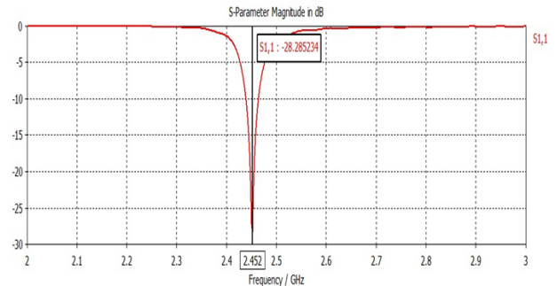
Fig. 2. Return loss response of Rectangular Patch Antenna.
