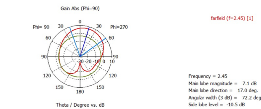
Fig. 8. Polar plot radiation pattern of Rectangular Patch Antenna.
