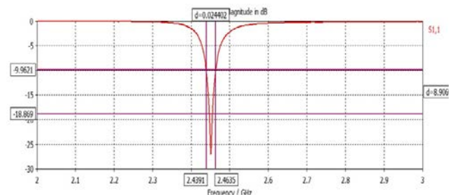
Fig. 5. Bandwidth calculation for Circular Patch Antenna.
