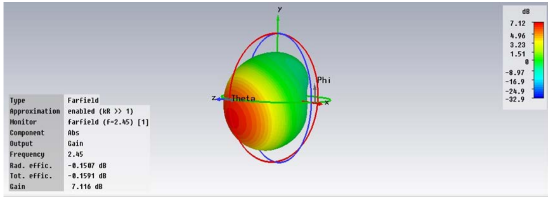
Fig. 6. 3D Radiation Pattern for Rectangular Patch Antenna
